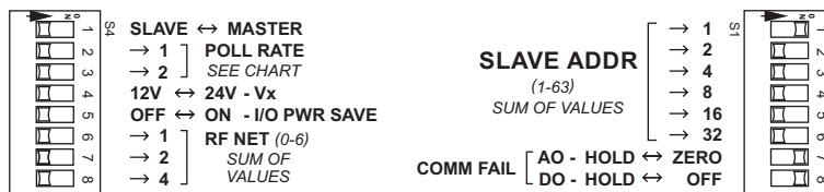
Figure 2 (Slave Unit Settings)
