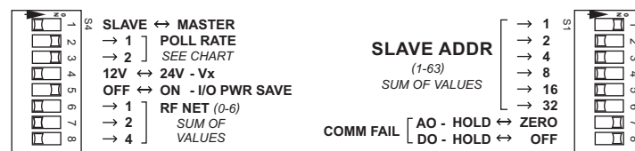
Figure 4 (Slave Unit Settings, Solar)
