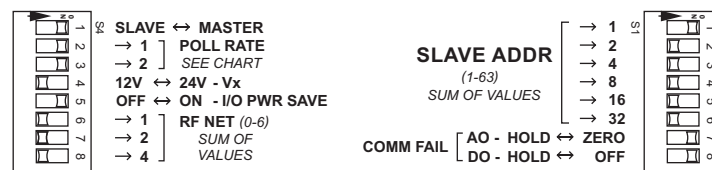
Figure 3 (Master Unit Settings, Solar)
